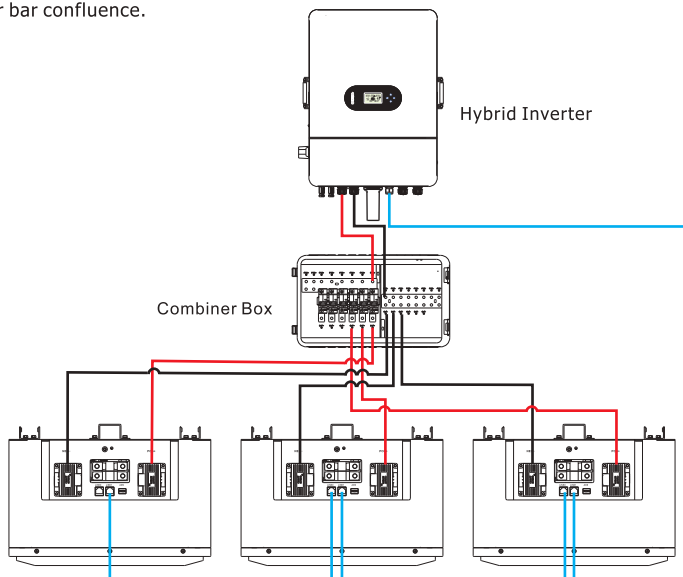
Figure 4-1 The parallel connection of three battery packs
