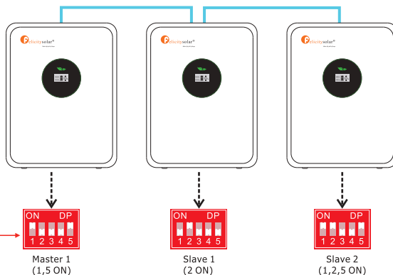
Example of three batteries in parallel
