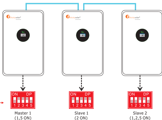
Example of three batteries in parallel
