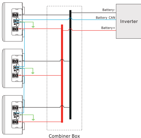
Figure 4-1 The parallel connection of three battery packs
