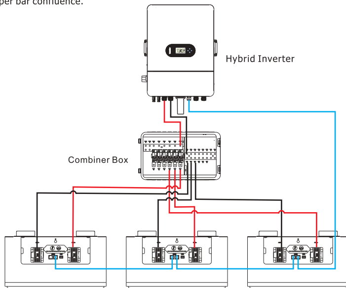
Figure 4-1 The parallel connection of three battery packs
