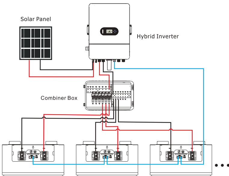
Figure 3-2 Multiple Battery Parallel System Connection Diagram
