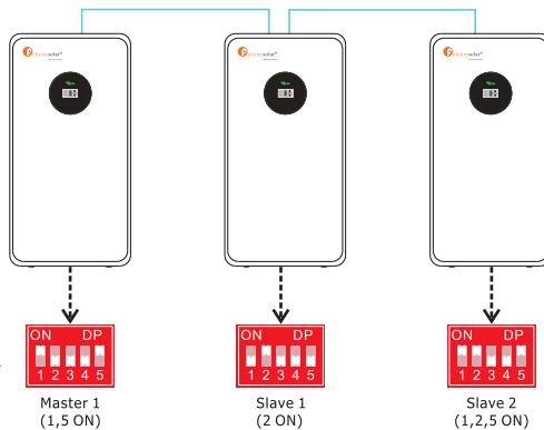
Example of three batteries in parallel
