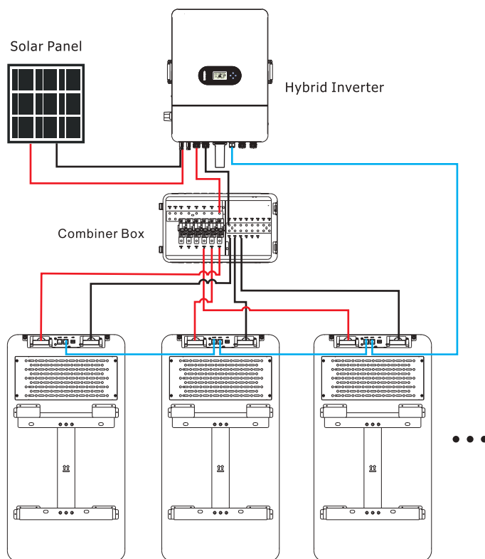
Figure 3-2 Multiple Battery Parallel System Connection Diagram
