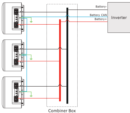
Figure 4-1 The parallel connection of three battery packs
