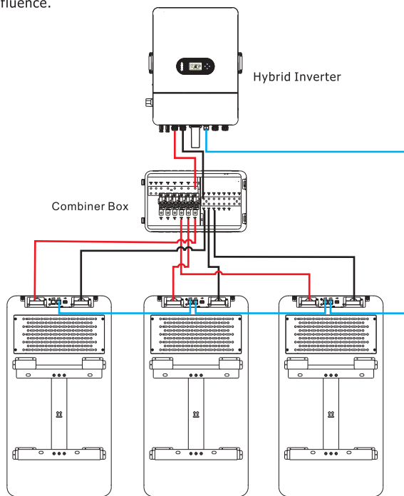
Figure 4-1 The parallel connection of three battery packs
