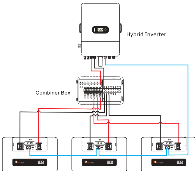
Figure 4-1 The parallel connection of three battery packs
