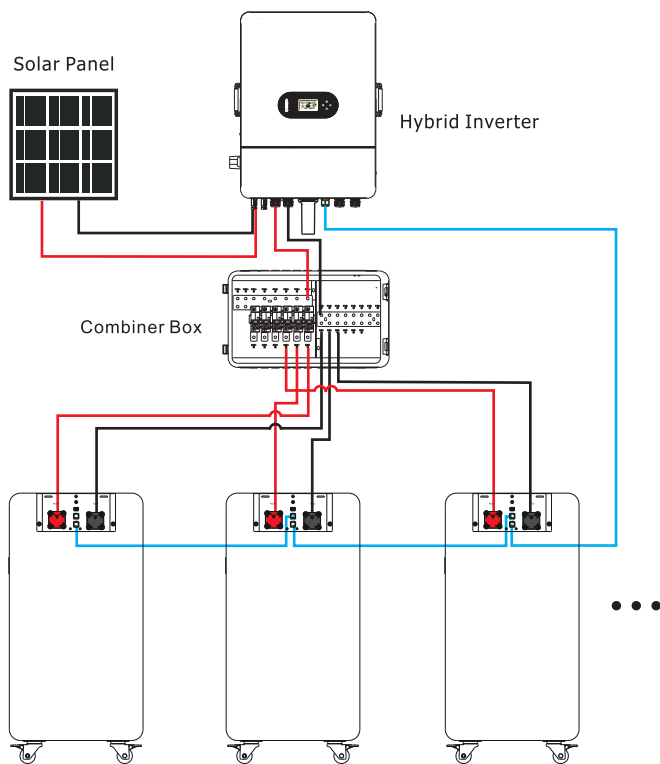
Figure 3-2 Multiple Battery Parallel System Connection Diagram
