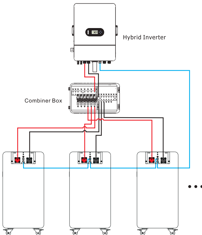
Figure 4-1 The parallel connection of three battery packs
