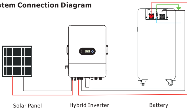
Figure 3-1 Single Battery System Connection Diagram
